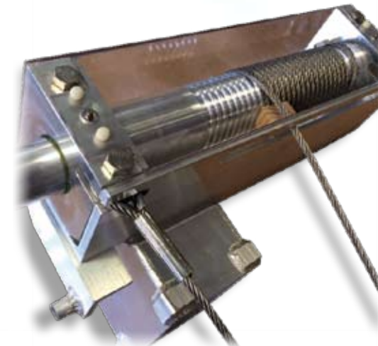
Solid Aluminum Deep Grooved Winder with Billet Bearings and a Lexan Safety Cover
